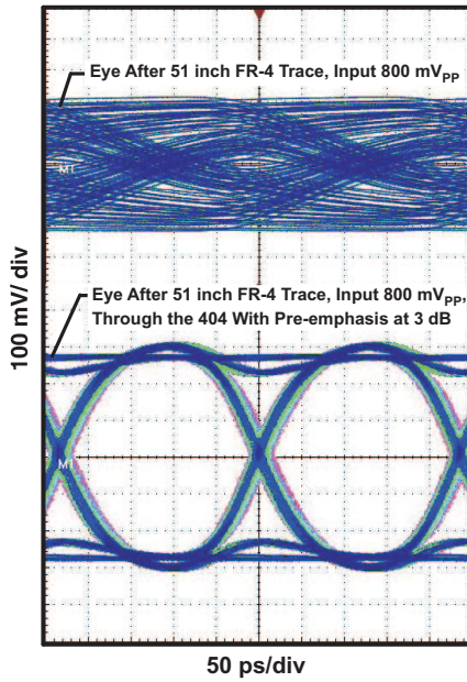
NOTE: 51 Inch (128.54 cm) Input Trace, dR = 4.25 Gbps; 2 7 -1 PRBS Figure 9. Data Input and Output Pattern
